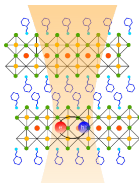
Figure 1: Schematic representation of the photogeneration of excitons in a 2D halide perovskite, formed of inorganic layers (PbI 6 octahedra) and large organic molecule (phenylethylammonium, in blue)
