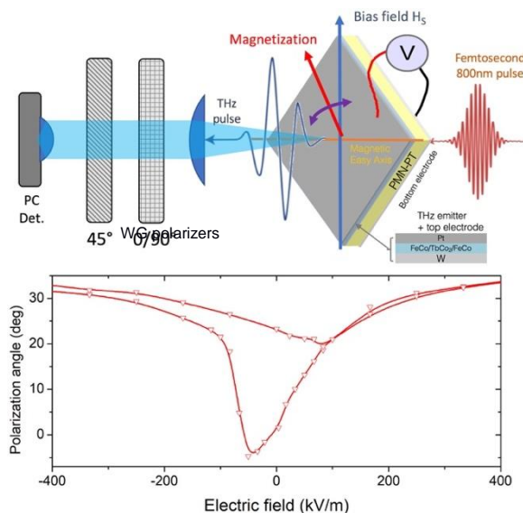
Figure 1 : Top : schematic representation of the magneto-electric spintronic emitter and characterization setup. Bottom: measured E-polarization angle with respect to the horizontal plane, as a function of the applied voltage on PMN-PT.
